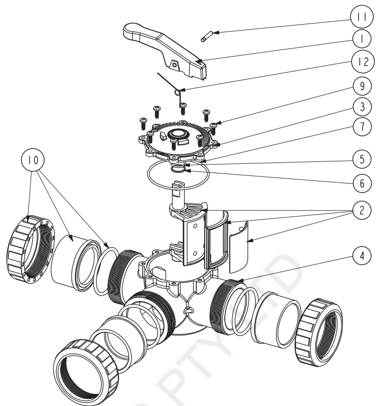
FPI Valve 65mm Threaded
