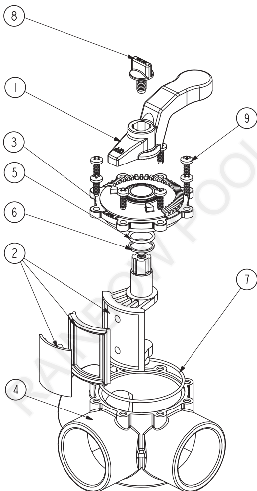
FPI Valve 50mm Actuated Slip Fit
