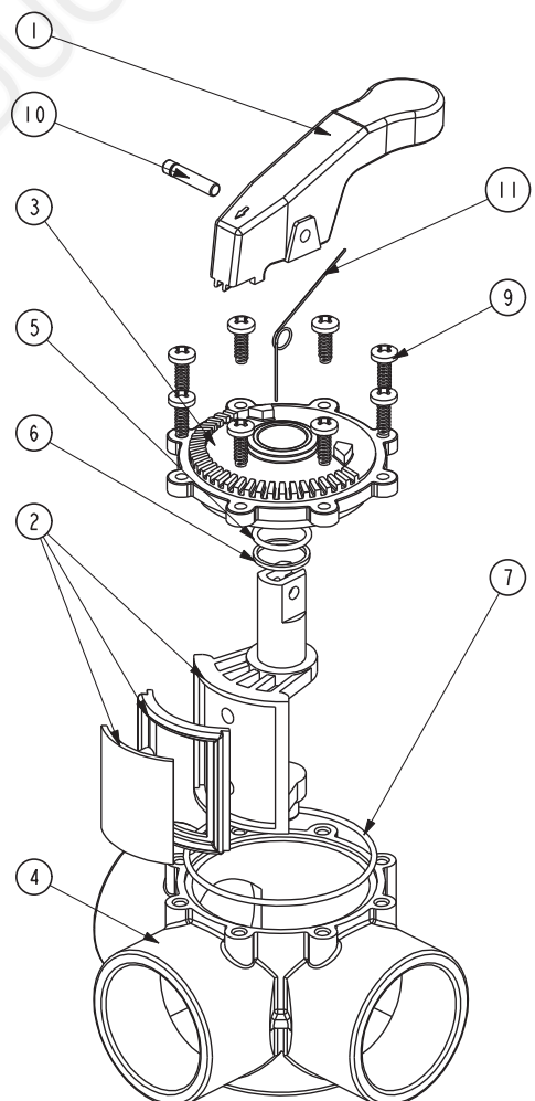
FPI Valve 50mm Slip Fit
