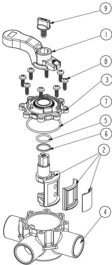
FPI Valve 25mm Slip Fit
