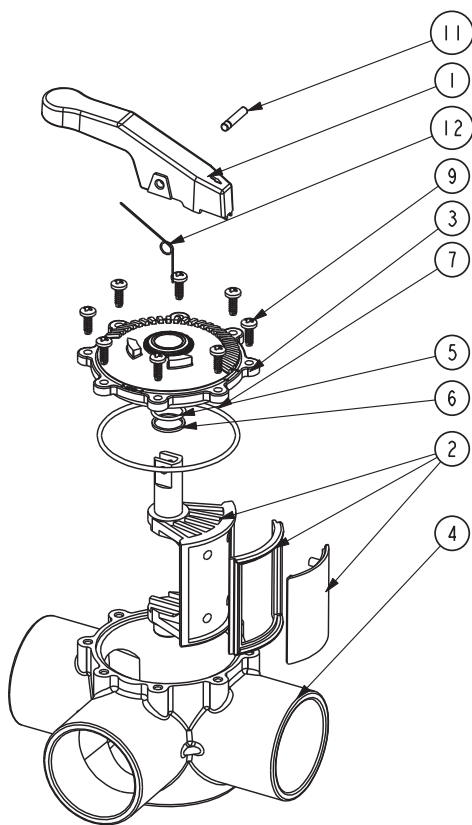
FPI Valve 65mm Slip Fit
