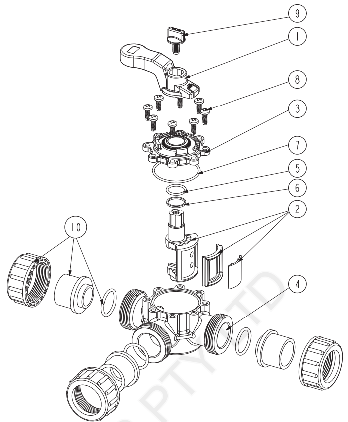
FPI Valve 25mm Threaded
