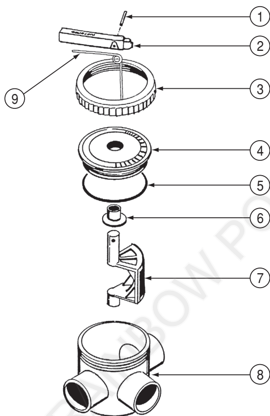
Fulflo 40mm Valve
