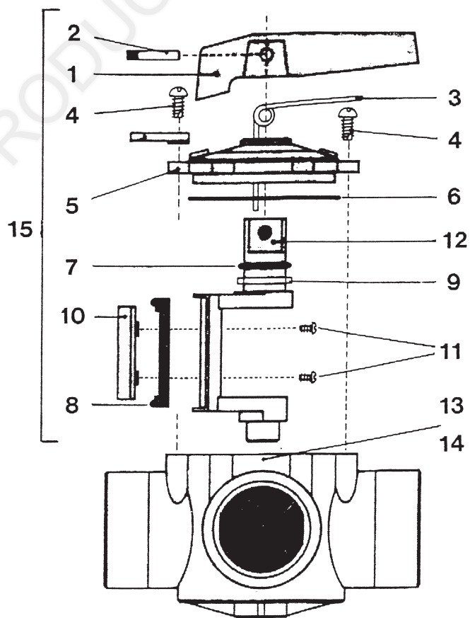
FPI 2 & 3 Way 40 mm Valve
