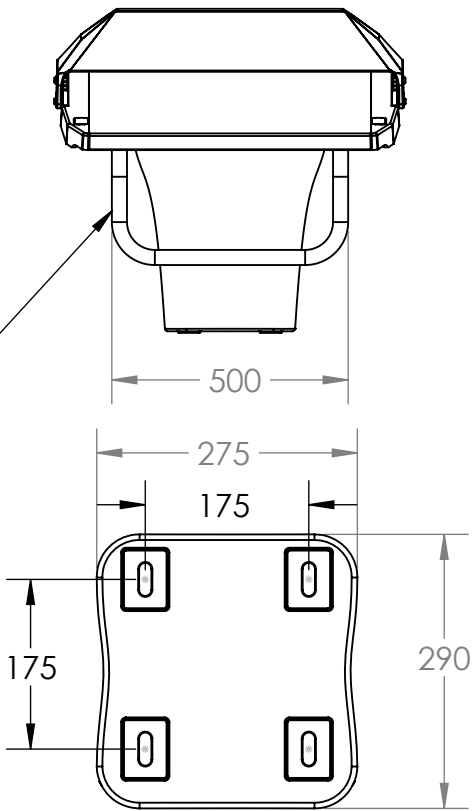
BOTTOM VIEW SCALE 1:8
