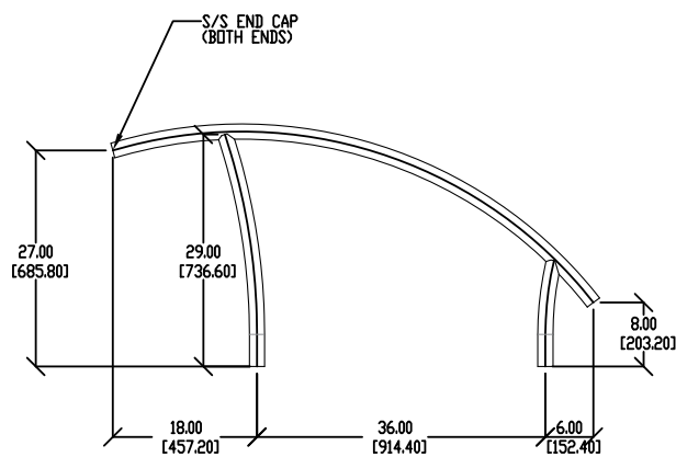
Deck-Mounted Hand Rail
