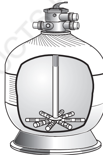
MICRON SAND FILTER
