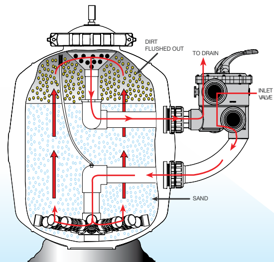
Backwash Mode
