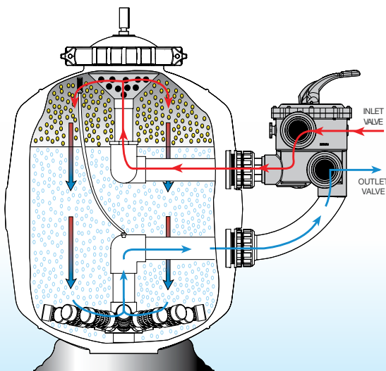
Filter Mode
