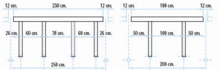
POSITION OF FIXINGS WHEN MEASUREMENT «L» IS OVER 500 mm.
