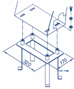
PLANT (Codes 28761, 28760 and 32700)
