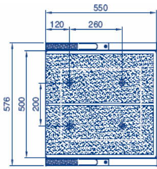
PLANT (Codes 28761, 28760 and 32700)
